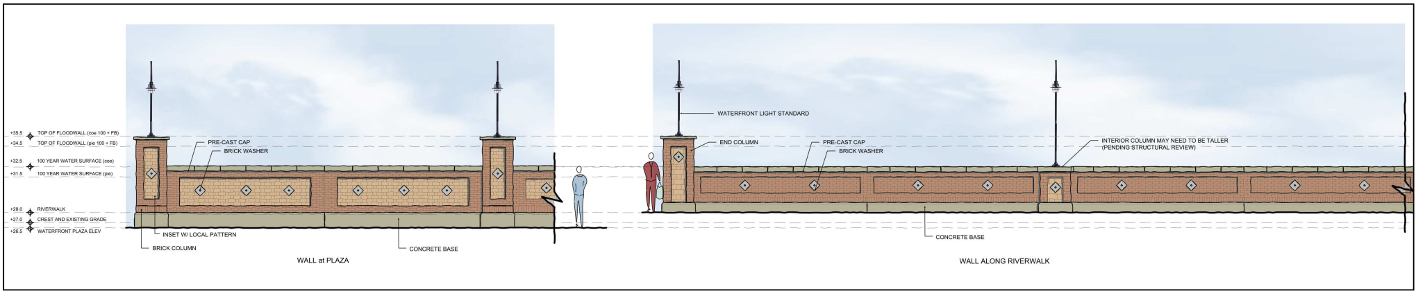
MASONRY WALL FRONT ELEVATION \frac{1}{4}'' = 1'-0''
