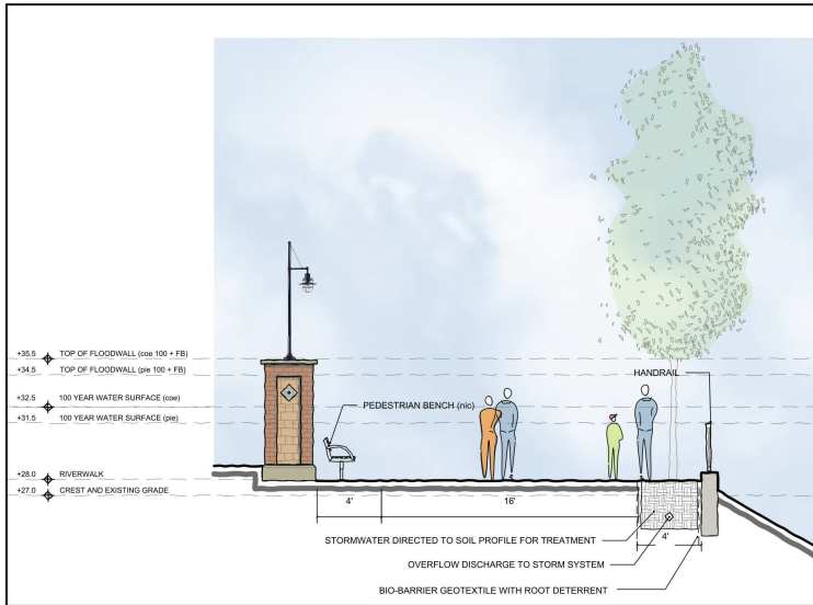
MASONRY WALL END ELEVATION \frac{1}{4}'' = 1'-0''
